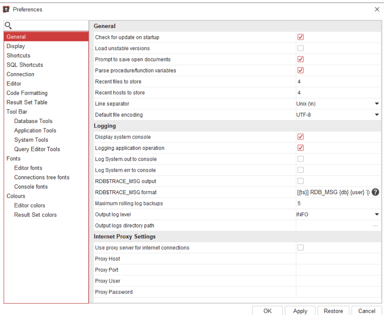
Img 18.4 — Preferences
