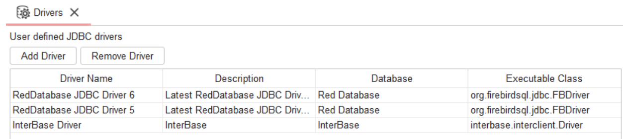
Img 18.1 — Drivers
