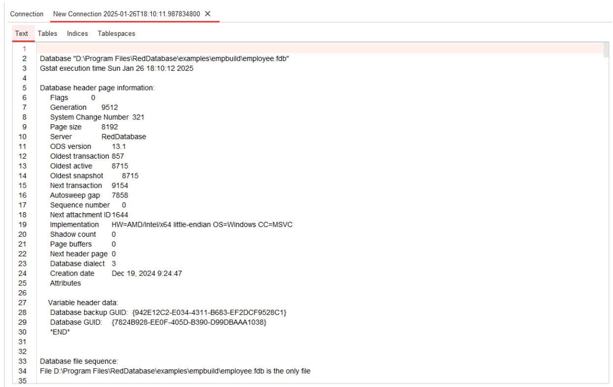
Img 10.2 — Statistics
